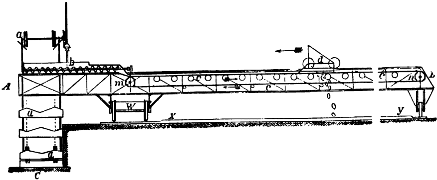
Fig. 400.—Mecke and Sanders' machine.
